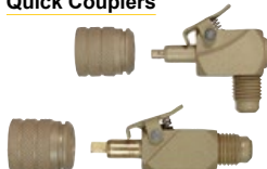
Quick disconnect couplers allow snap connection to the system to minimise refrigerant loss
